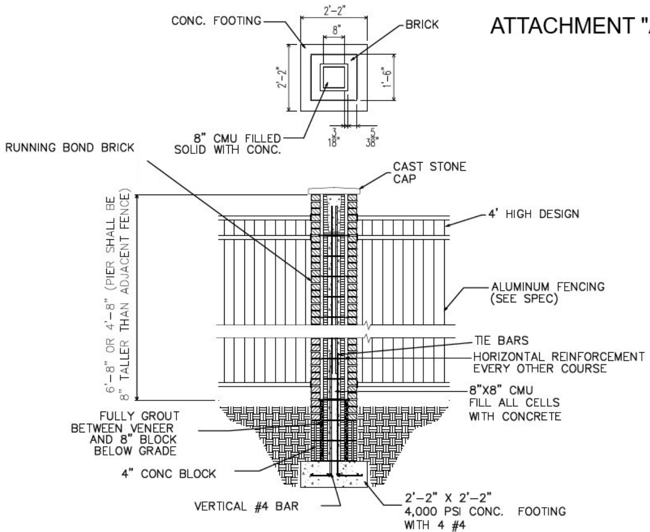
FENCE PIER PLAN & SECTION NOT TO SCALE
