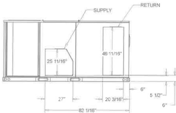
BACK VIEW OF UNIT DIMENSION DRAWING
