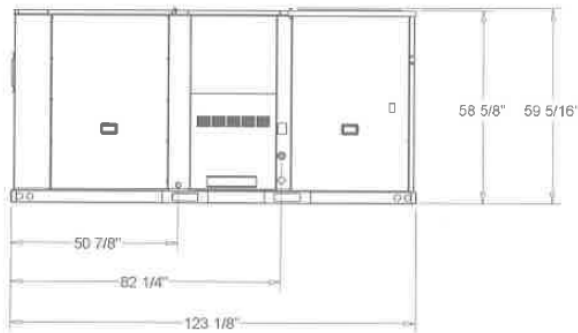
FRONT VIEW OF UNIT DIMENSION DRAWING
