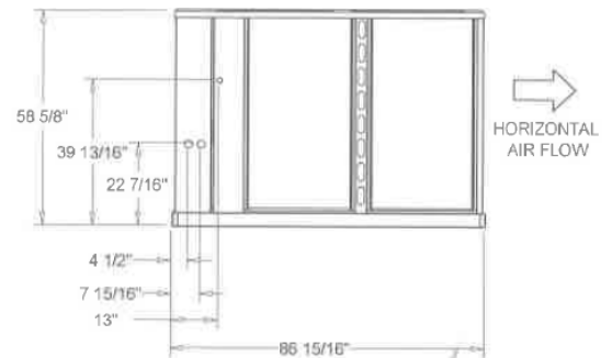
RIGHT SIDE VIEW OF UNIT DIMENSION DRAWING
